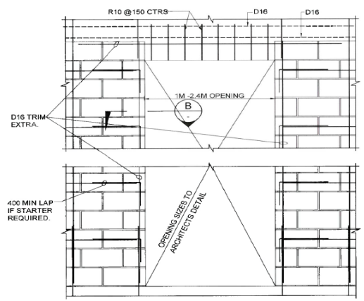
TYPICAL DOOR OPENING DETAIL
