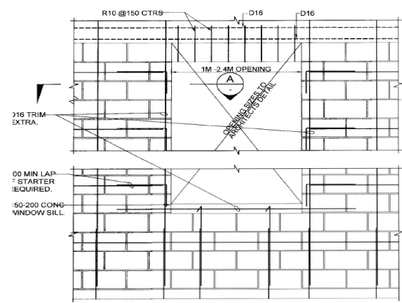
TYPICAL WINDOW OPENING DETAIL
