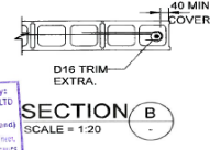
TYPICAL DOOR OPENING DETAIL
