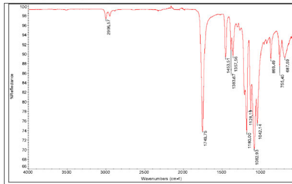
Fig.1: FTIR spectrum of original sample
